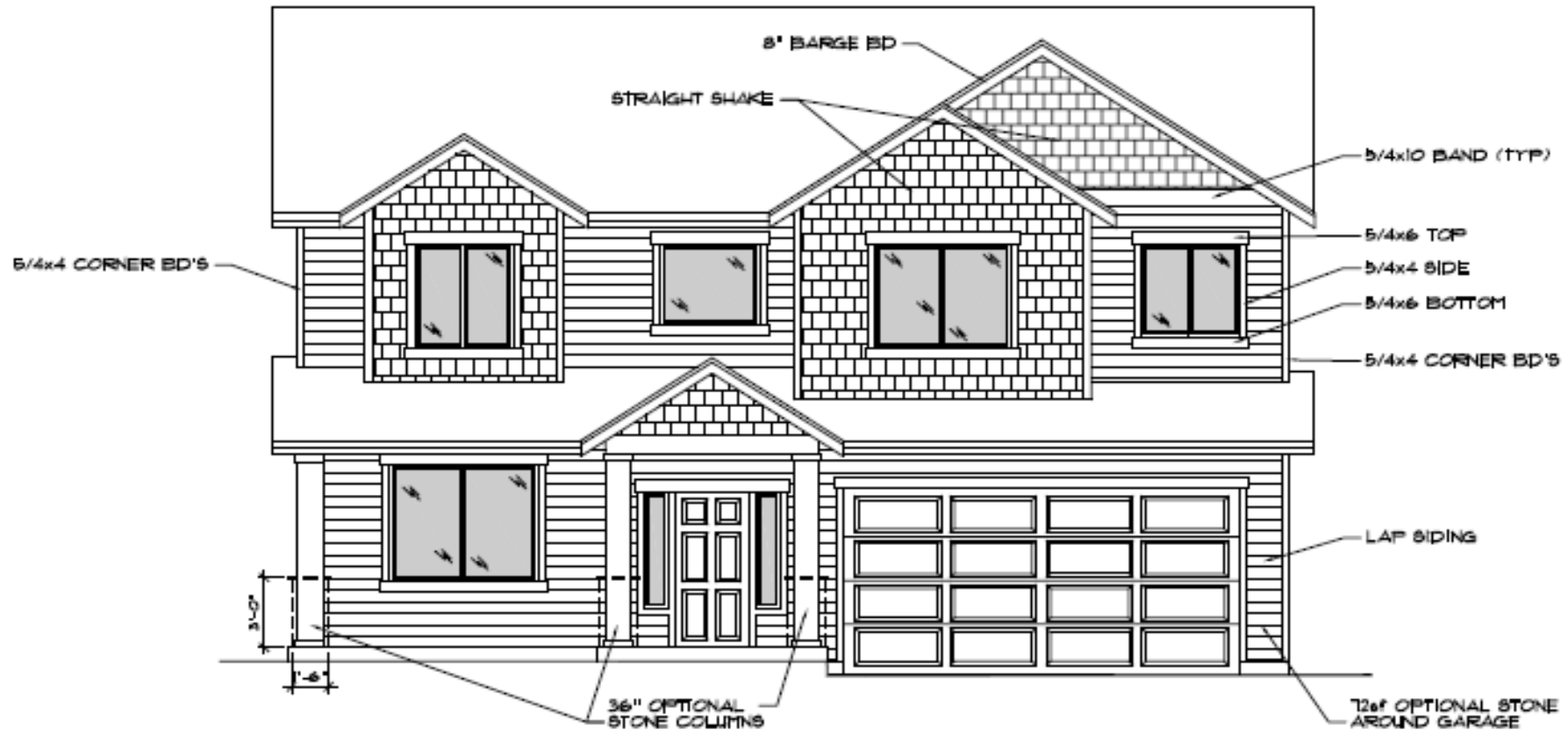
ELEVATION "A" TRIM 1
